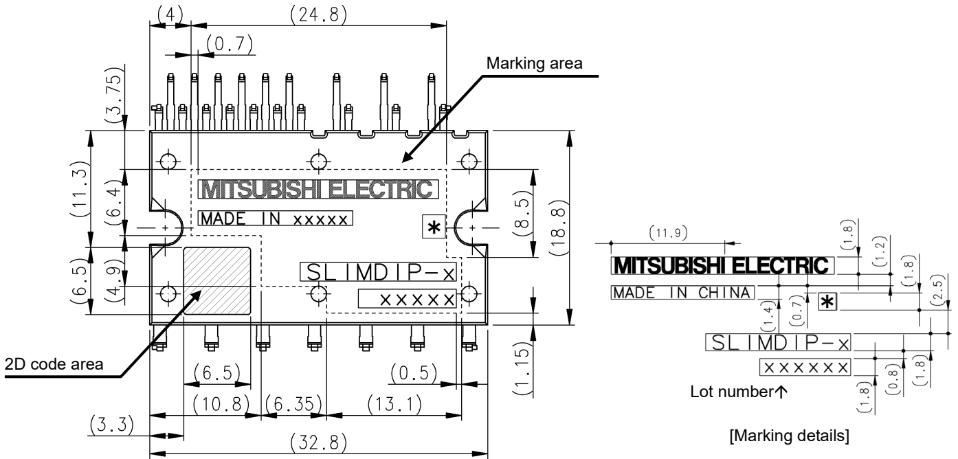
Fig.2-3-4 Laser marking view
