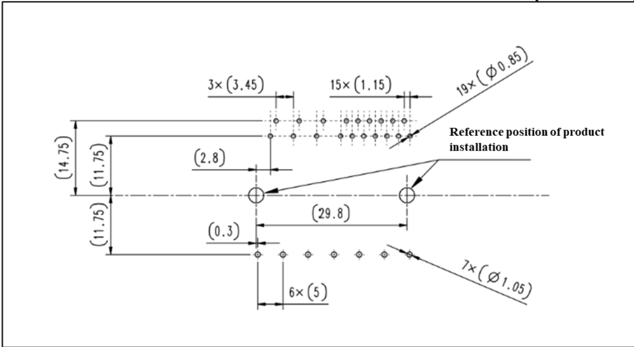
Fig.2-3-3 PCB through-hole pattern of SLIMDIP (Reference Figure)
