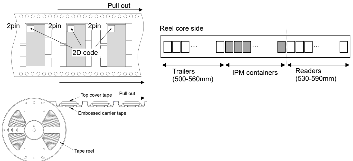
Fig.5-1-3 Carrier tape packing specifications
