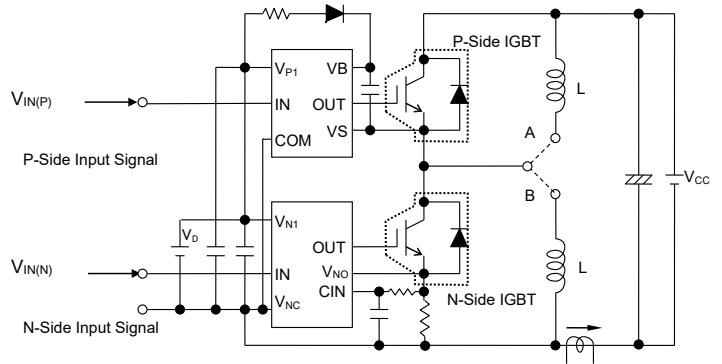
Fig.2-1-4 Evaluation circuit (inductive load) *Short A for N-side switching, or short B for P-side switching.
