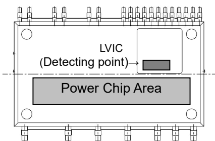
Fig.2-2-7 Temperature detecting point
